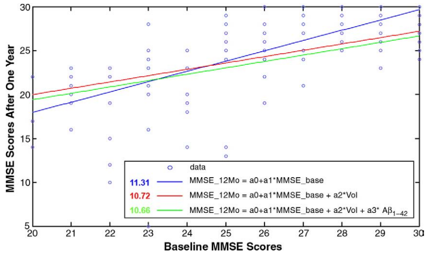
Fig. 12. Predicting later cognitive decline from baseline measures of MMSE, ventricular volumes and the A\beta_{1-42} biomarker using least-squares regression models. MMSE_{12Mo} , MMSE_{base} , Vol and A\beta_{1-42} denote MMSE scores after a one-year follow-up interval, the baseline MMSE score, ventricular volumes and A\beta_{1-42} protein levels, respectively. The values shown in the legend represent the mean square of the deviations of the data from the predictive models, showing that prediction errors were successively reduced (but only by about 5%) as each more invasive measure was added to the predictive model.
